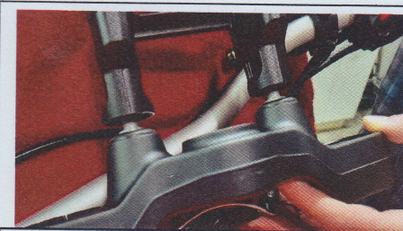
As you Loosen the 15mm perch nuts, the perches un-thread and rise upward and off. Un-do each side a little at a time.
